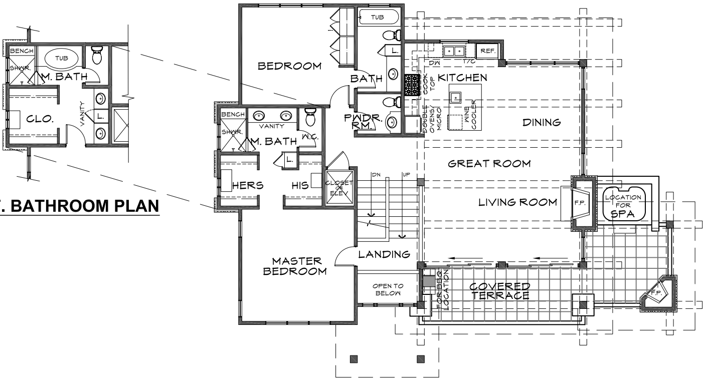
UPPER LEVEL FLOOR PLAN
